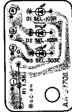
6) LED P.C BOARD AA-5270B
