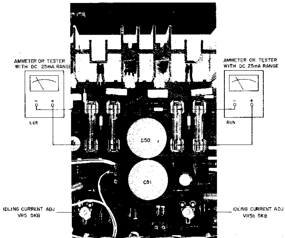
Fig. 22 Main Amplifier Adjustment (AA-1125)
