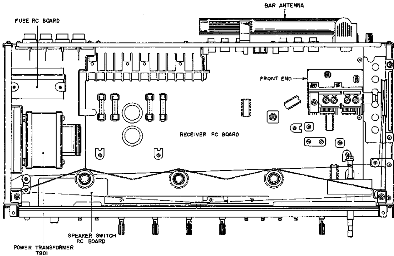
Fig. 5 Top View
