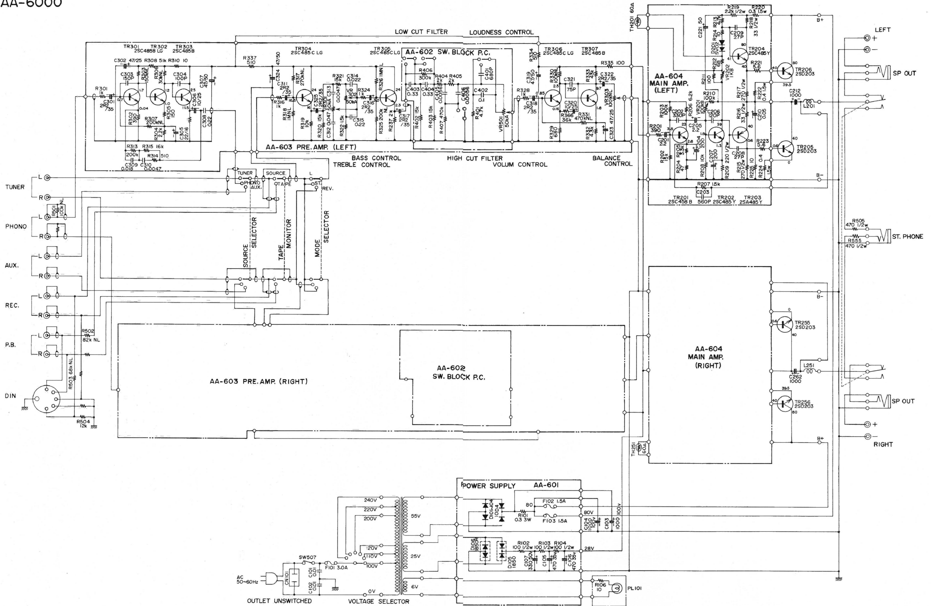
AA-6000 SCHEMATIC DIAGRAM 13818381
