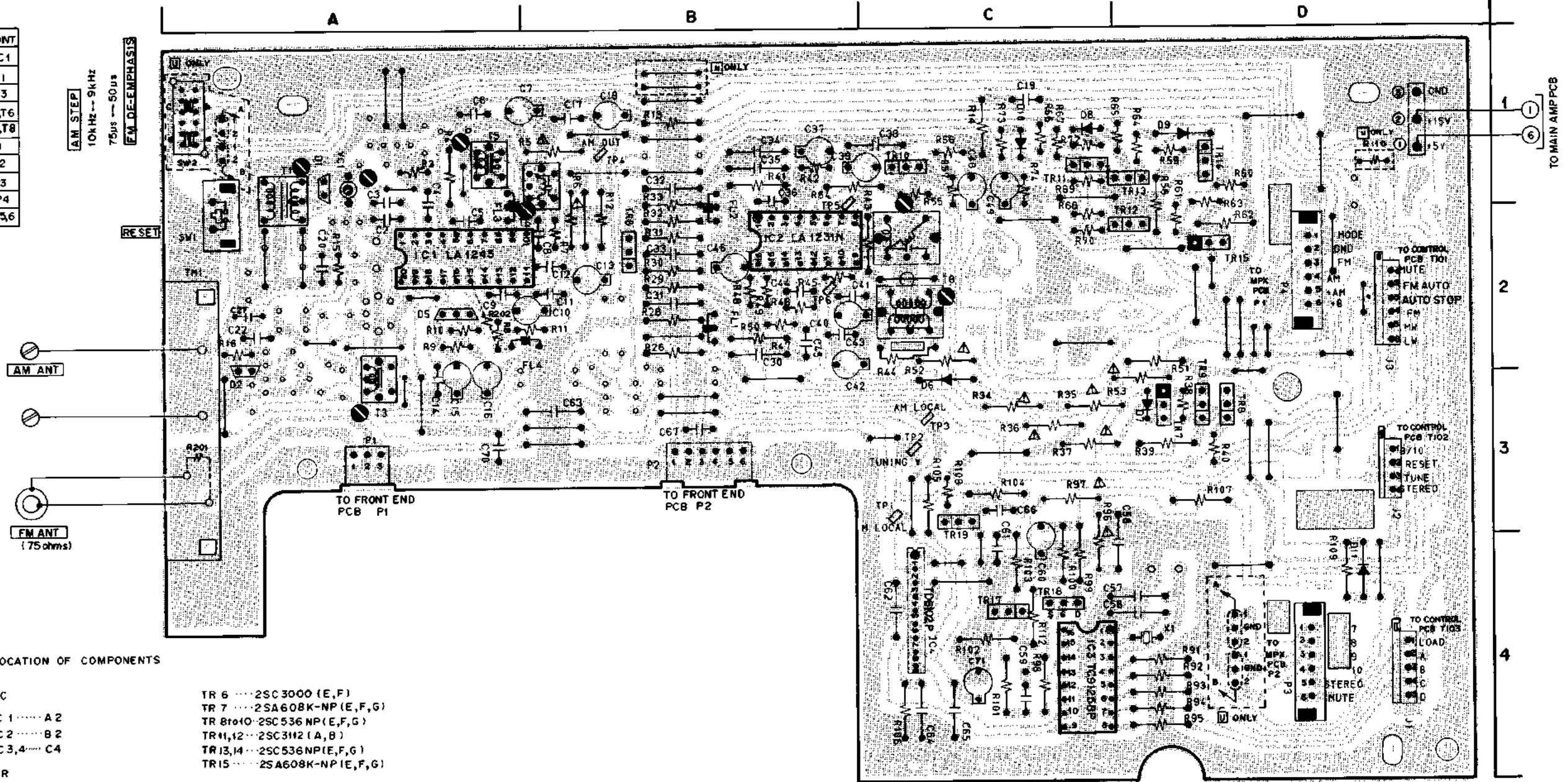
TUNER PCB A1007B502A
