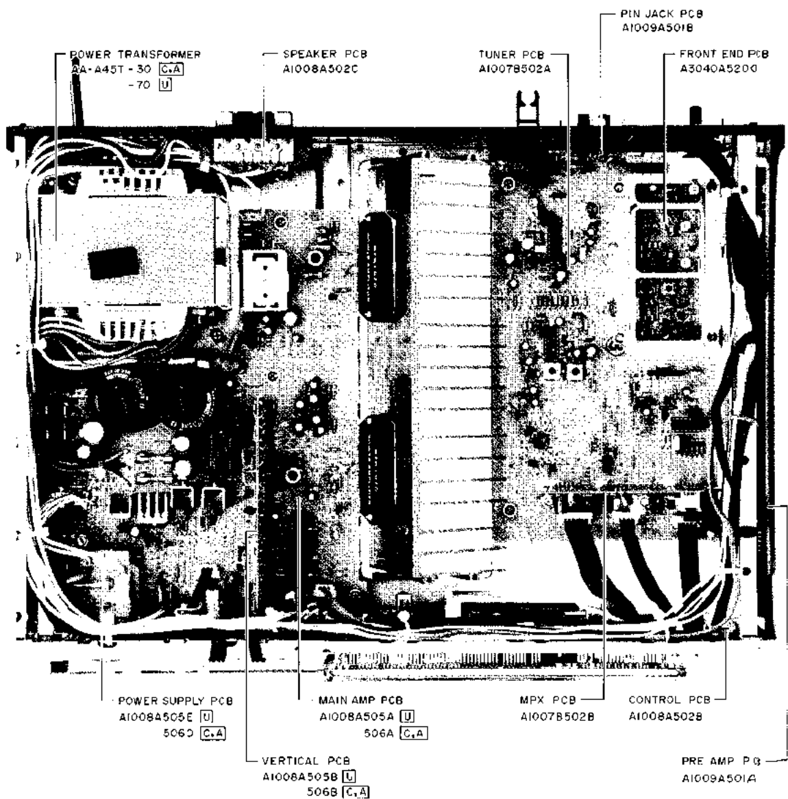
Fig. 4-2 Top View
