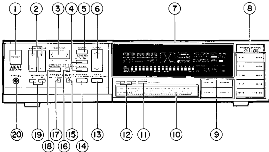
Fig. 3-1 Front View
