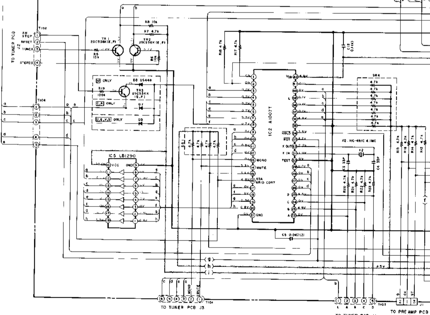
CONTROL PCB A1008A502B
