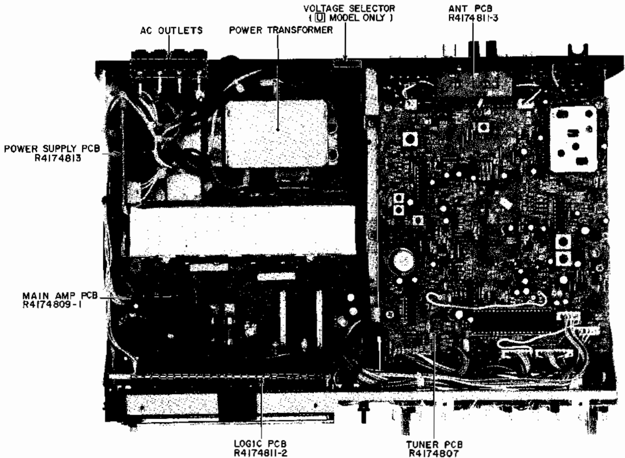
Fig. 4-2 Top View
