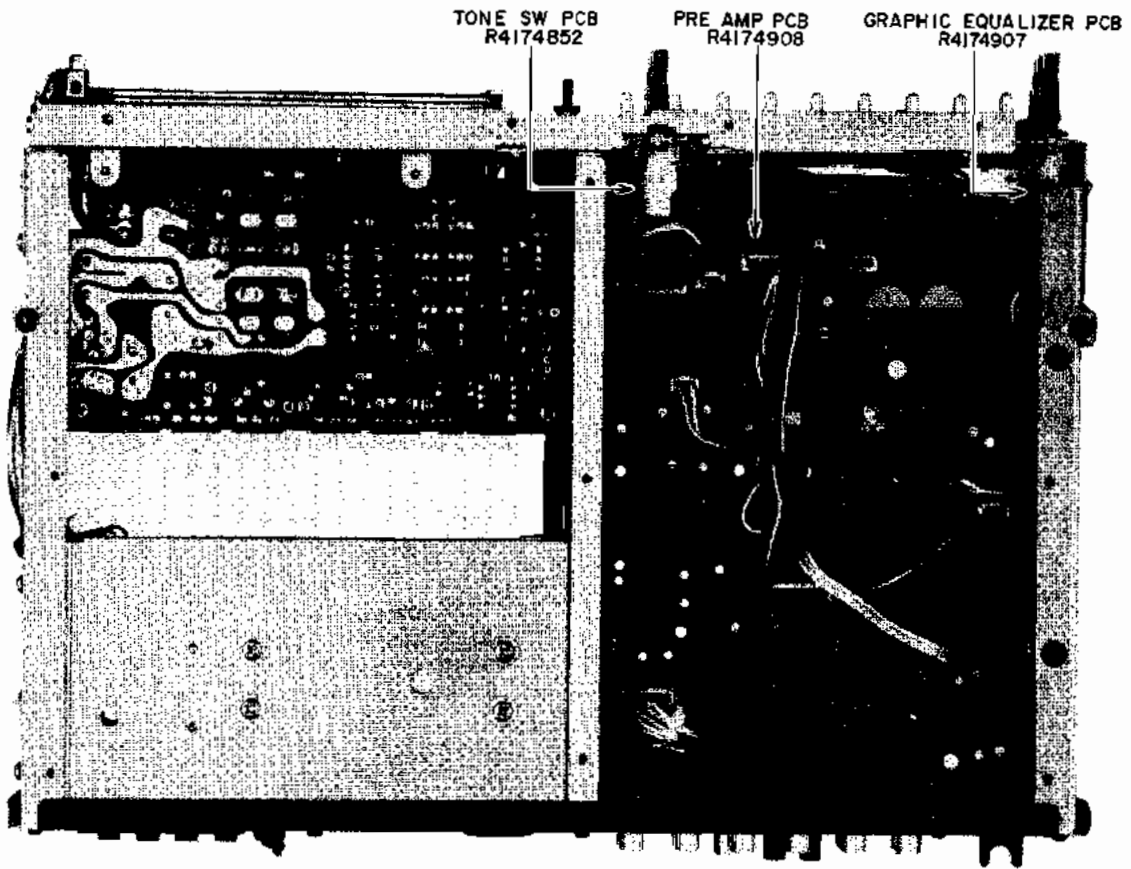
Fig. 4-3 Bottom View
