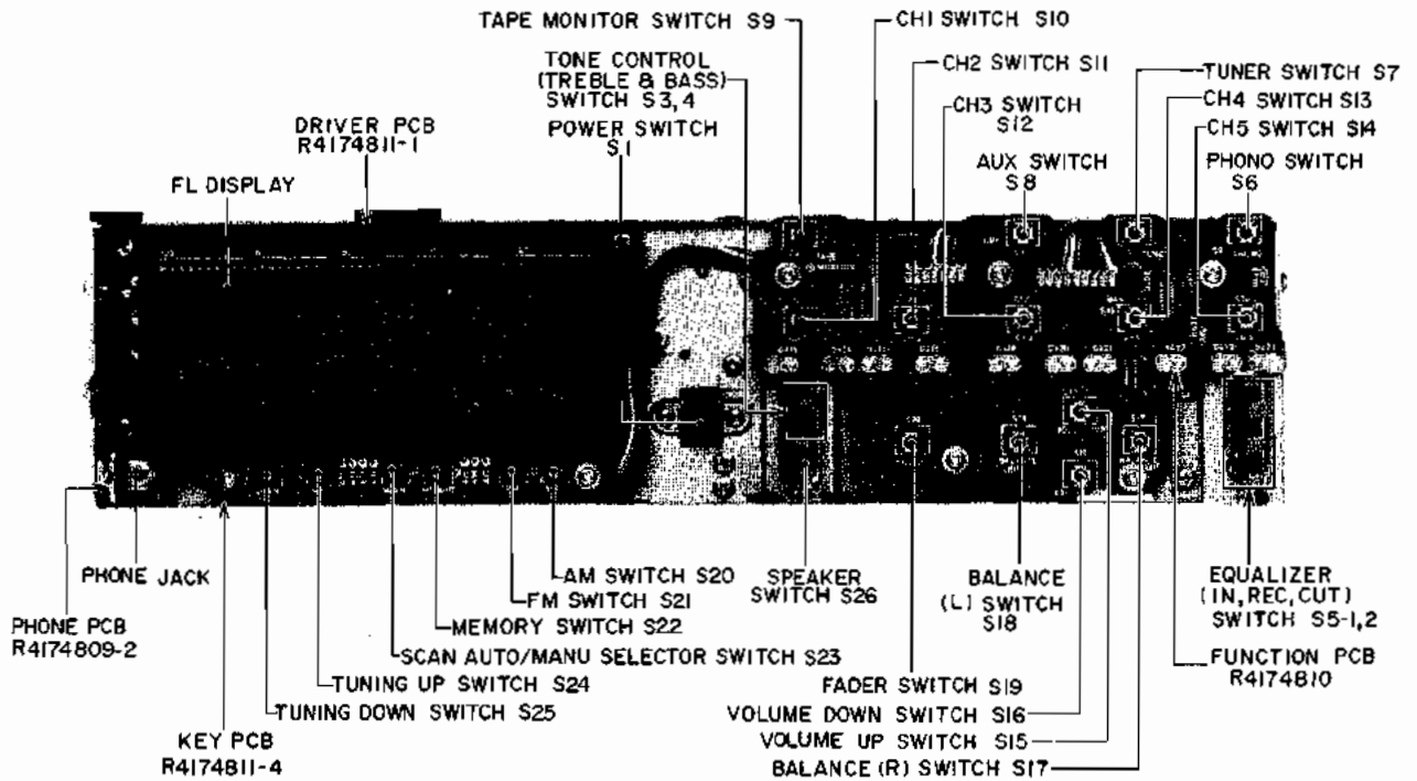
Fig. 4-1 Front View
