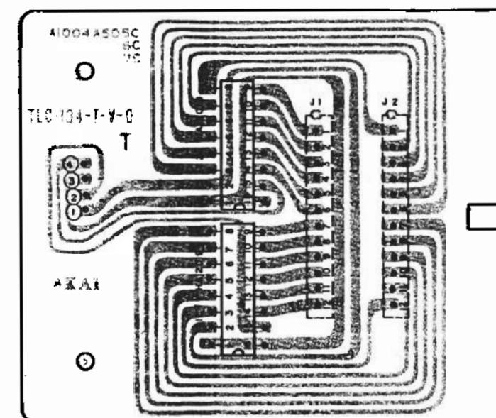
BAR METER PCB (U) A1004A505C (C, A) A1004A506C (E, B, S) A1004A507C
