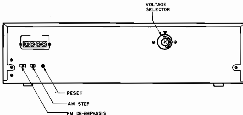
Fig. 3-6 Rear View
