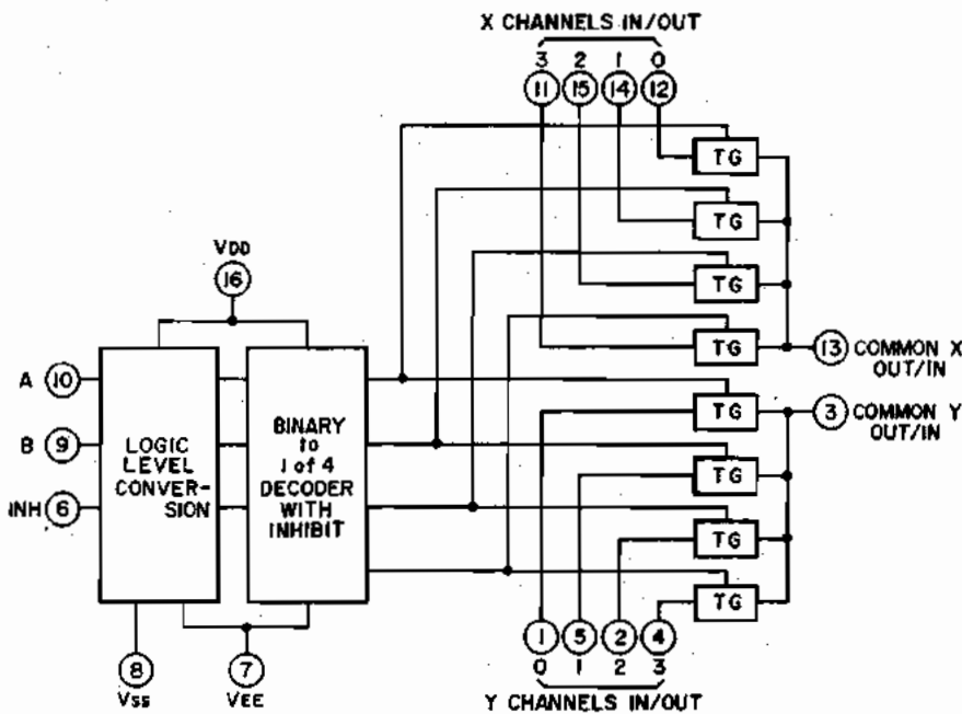
SCHEMATIC DIAGRAM AA-R22/L, AA-R32/L, AA-R42
