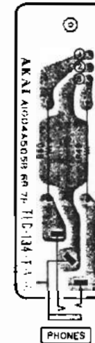
HEAD PHONE PCB (U) A1004A505B (C,A) A1004A506B (E,B,S) A1004A507B
